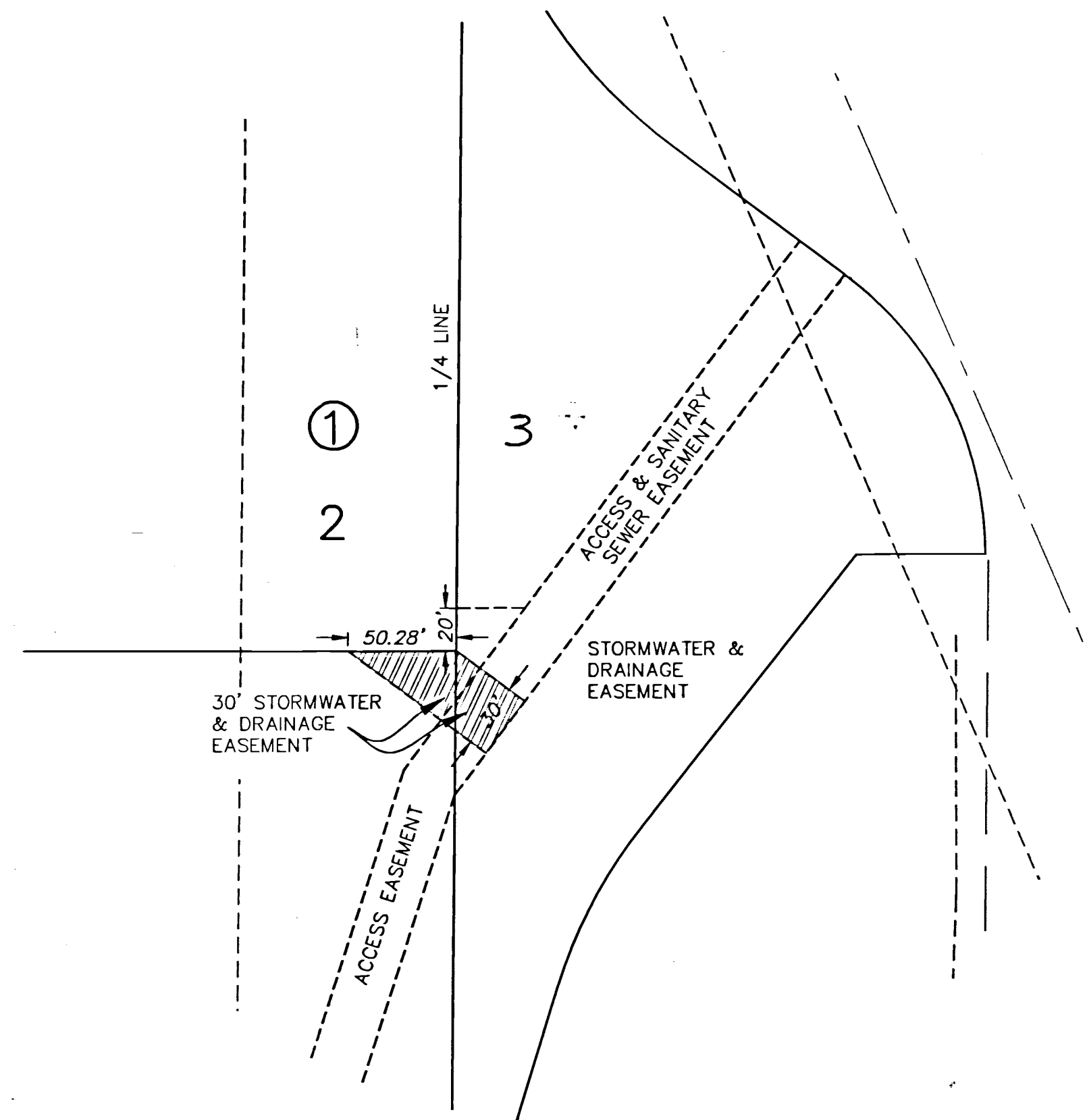
STORMWATER & DRAINAGE DETAILS (NOT TO SCALE)
