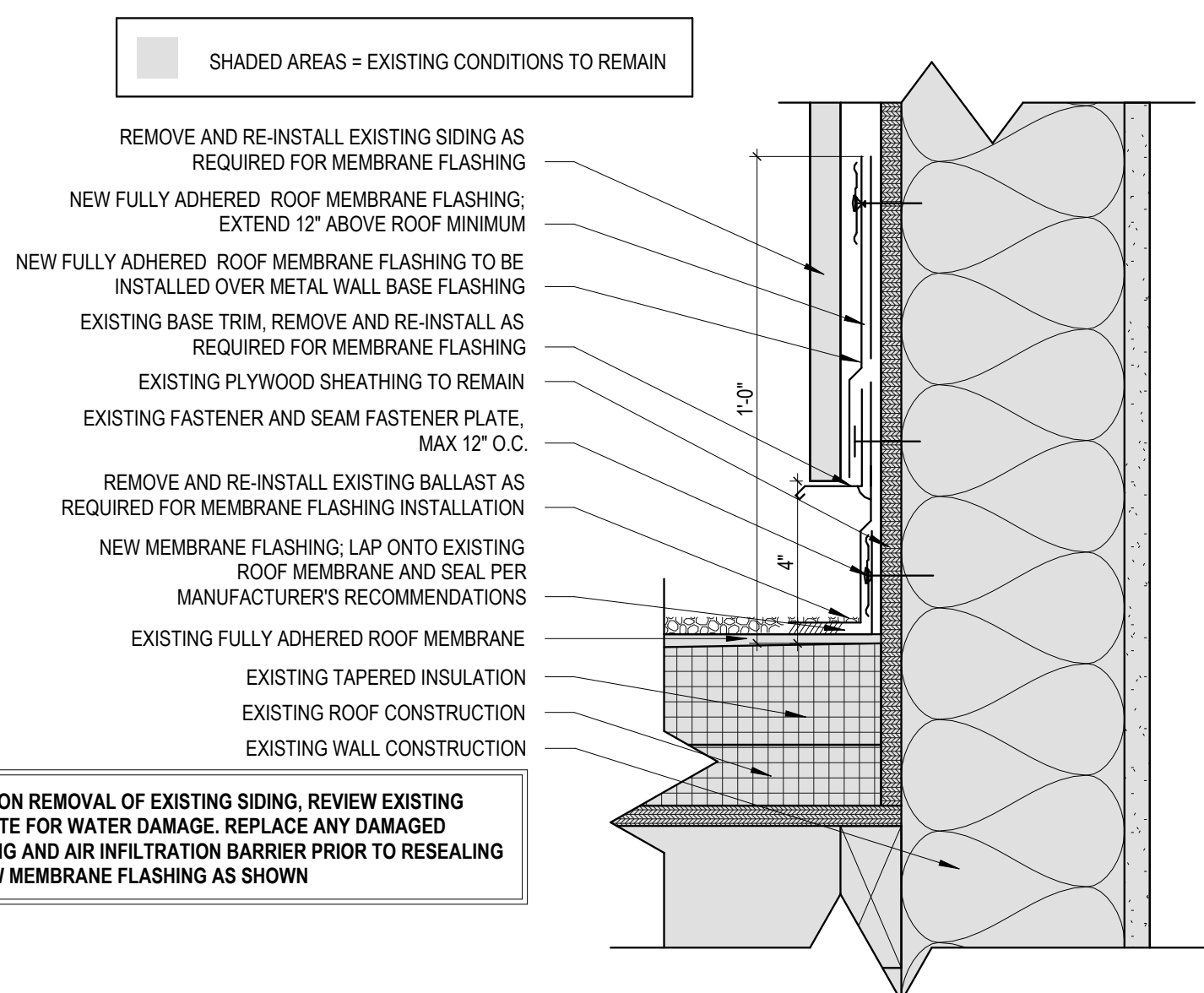
6 Roof to Wall Detail Scale: 3\"/>
