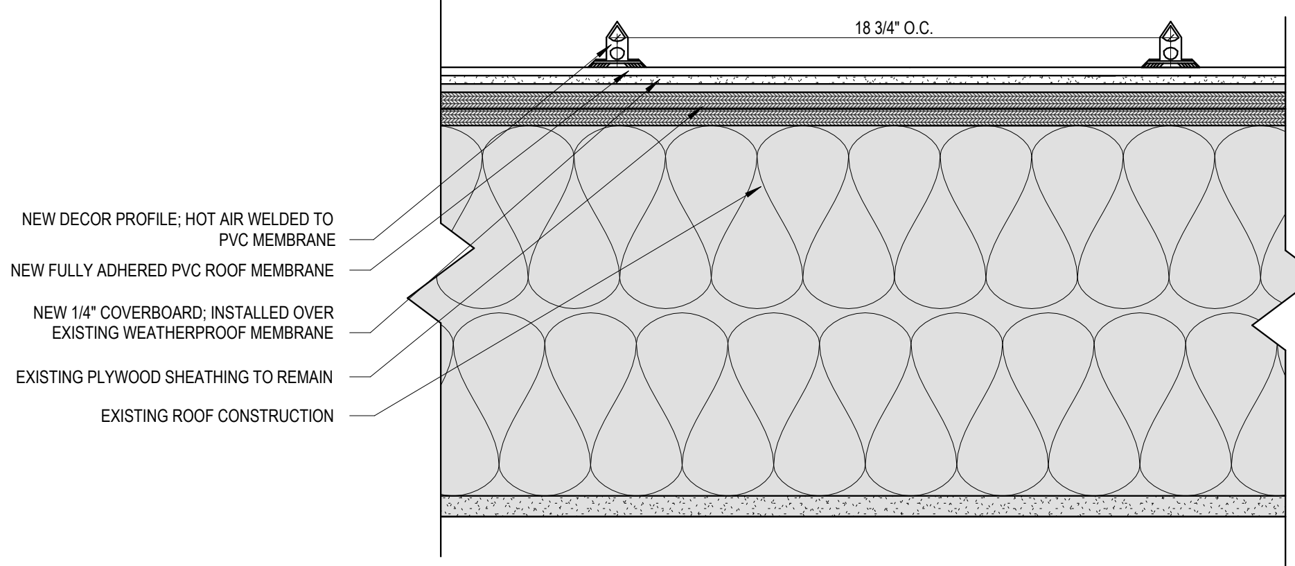
2 Typical Roof Section Scale: 3\"/>
