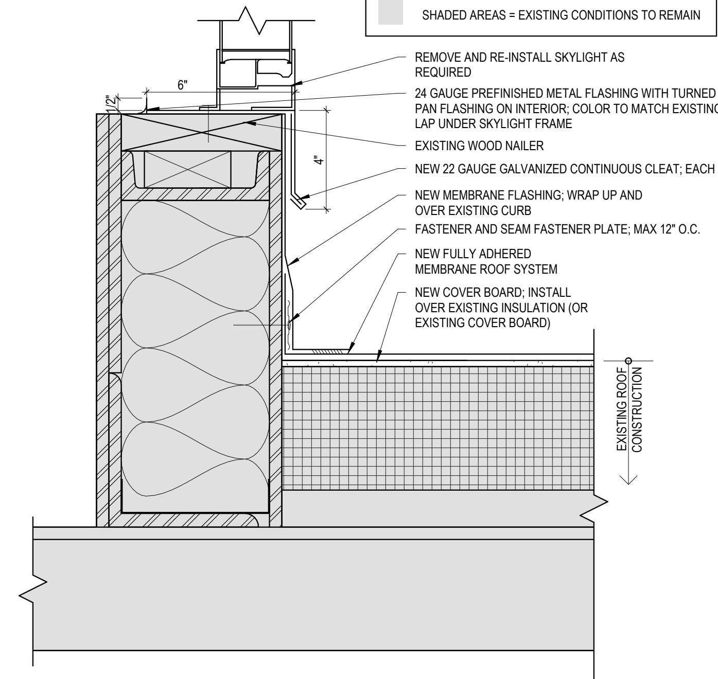
3 Roof Curb at Skylight Detail Scale: 3" = 1'-0"
