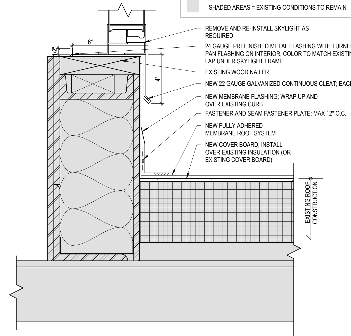
3 Roof Curb at Skylight Detail Scale: 3" = 1'-0"
