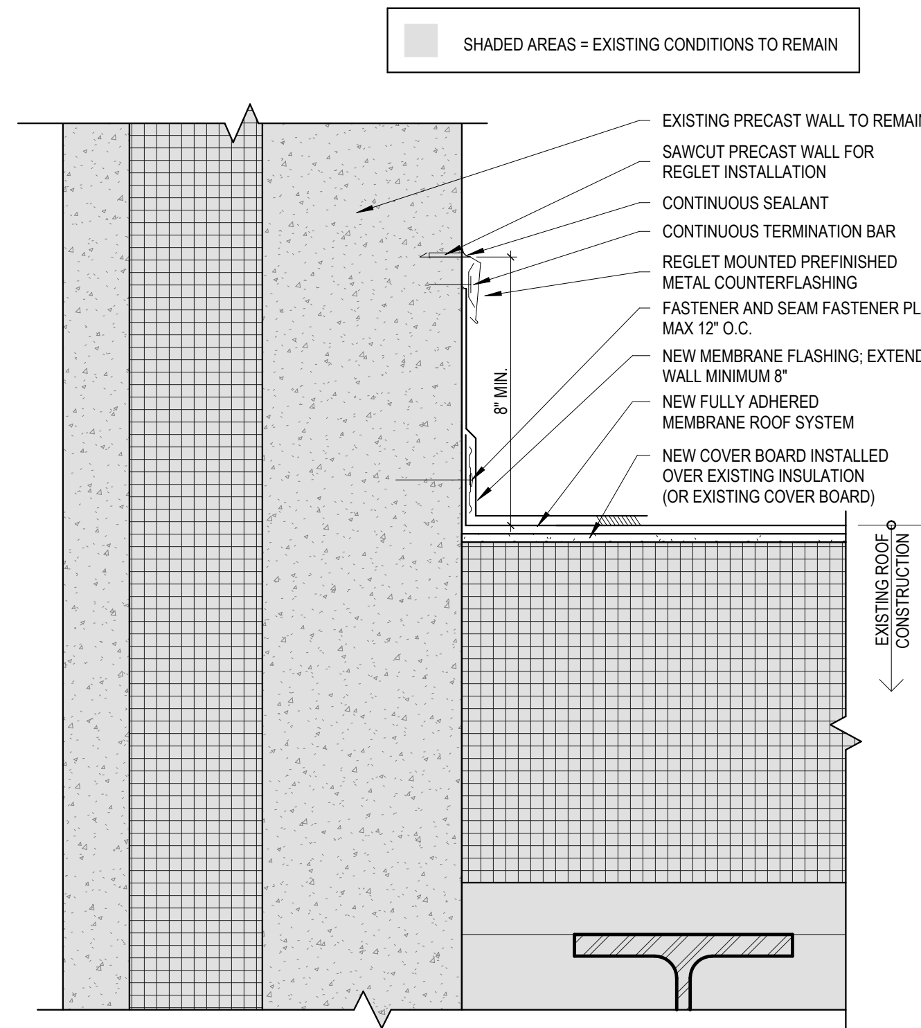
3 Roof Counterflashing Detail Scale: 3/4" = 1'-0"
