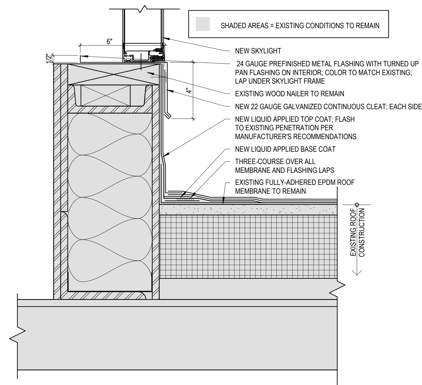
6 Skylight Roof Curb Detail - Alt. Bid #1 Scale: 3" = 1'-0"
