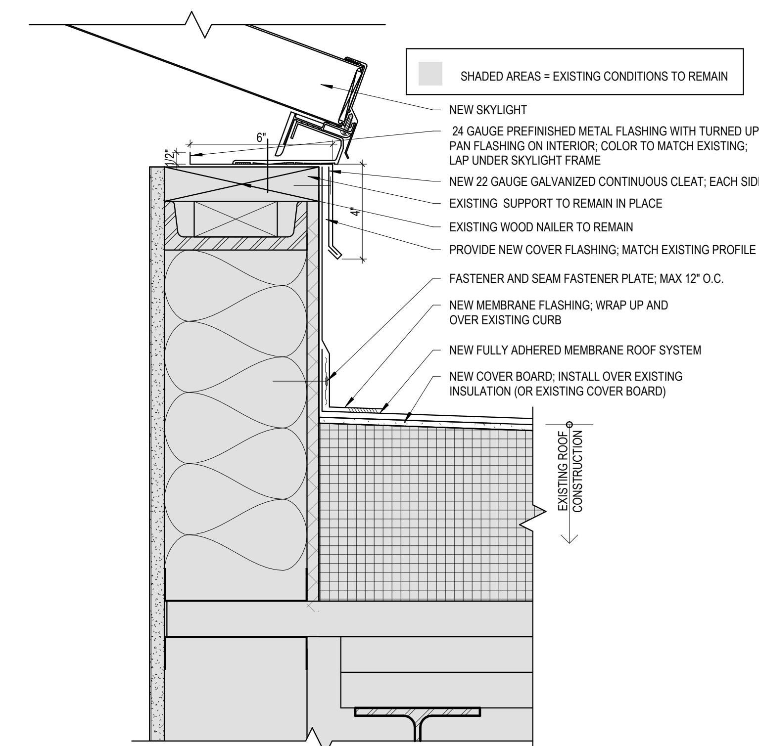
8 Skylight Roof Curb Detail - Alt. Bid #1 Scale: 3" = 1'-0"
